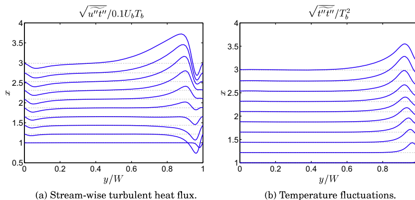
Fig. 20. \overline{u''t''} and \overline{t''t''} profiles across the channel at different heights.
