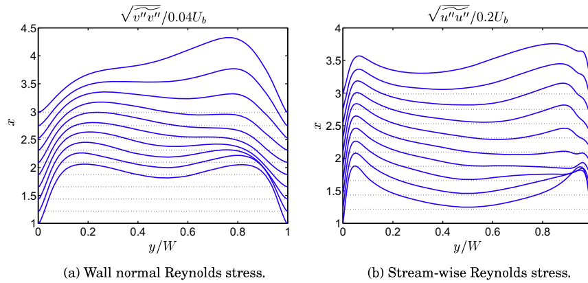
Fig. 19. \overline{v''v''} and \overline{u''u''} profiles across the channel at different heights.
