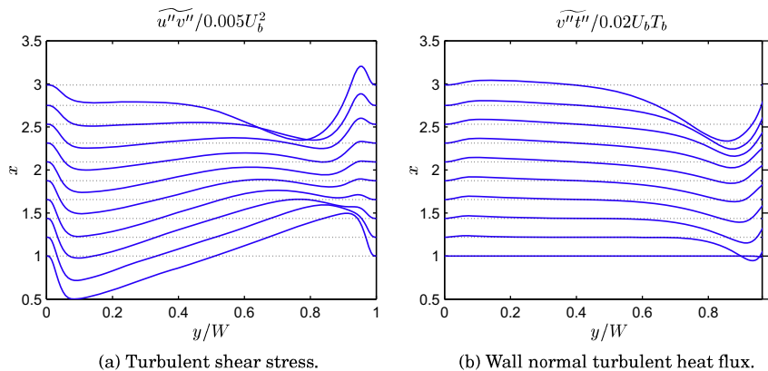
Fig. 18. \overline{u''v''} and \overline{v''t''} profiles across the channel at different heights.
