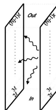
Fig. 2. Schematic diagram of the radiation heat transfer in the channel.
