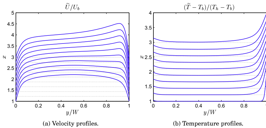
Fig. 17. Velocity and temperature profiles across the channel at different heights.
