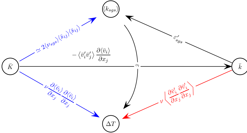
Figure Q.3: Transfer of kinetic turbulent energy. \bar{K} = \frac{1}{2}\langle\bar{v}_i\rangle\langle\bar{v}_i\rangle and \bar{k} = \frac{1}{2}\langle\bar{v}'_i\bar{v}'_i\rangle denote time-averaged kinetic and resolved turbulent kinetic energy, respectively. \Delta T denotes increase in internal energy, i.e. dissipation. The cascade process assumes that the term in red is negligible (see also Fig. 8.2). The terms in blue show viscous and the SGS dissipation of the mean flow which is not included in the cascade process.
