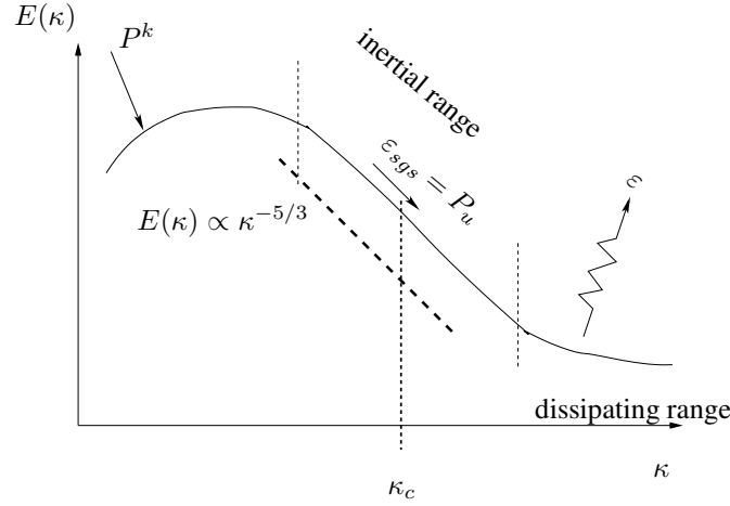
Figure V.2: Energy spectrum.
