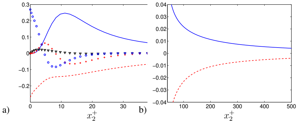
a) Zoom near the wall; b) Outer region. —: P^k ; - - - : -\epsilon ; \nabla : -\overline{\partial v' p} / \partial x_2 ; + : -\overline{\partial v'_2 v'_i v'_i} / 2 / \partial x_2 ; \circ : \nu \partial^2 k / \partial x_2^2 .
