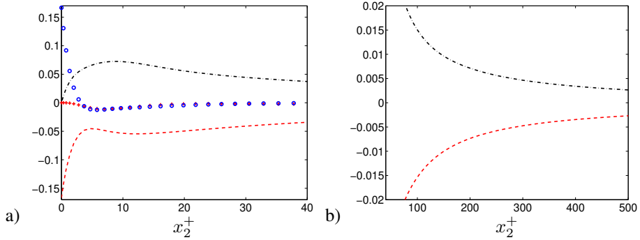
Figure 9.5: Channel flow at Re_\tau = 2000 . Terms in the \overline{v_3''} equation scaled by u_\tau^4/\nu . a) Zoom near the wall; b) Outer region. DNS (Direct Numerical Simulation) data [15, 16]. -\text{---} : -\varepsilon_{33} ; -\text{- - -} : \Pi_{33} ; + : -\partial(\overline{v_2' v_3''})/\partial x_2 ; \circ : \nu \partial^2 \overline{v_3''}/\partial x_2^2 .
