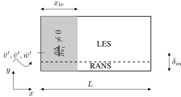
Figure 26.2: Boundary layer flow.
