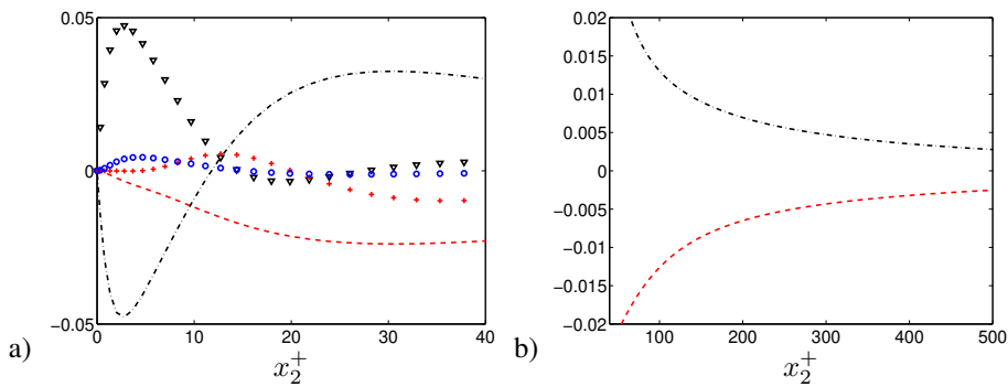
Figure 9.4: Channel flow at Re_\tau = 2000 . Terms in the \overline{v'^2} equation scaled by u_\tau^4/\nu . a) Zoom near the wall; b) Outer region. DNS (Direct Numerical Simulation) data [15, 16]. -\text{---} : -\varepsilon_{22} ; \nabla : -2\overline{v'_2 p'}/\partial x_2 ; \text{---}\blacksquare\text{---} : \Pi_{22} ; + : -\partial(\overline{v'_2 v'^2_2})/\partial x_2 ; \circ : \nu\partial^2 \overline{v'^2_2}/\partial x_2^2 .
