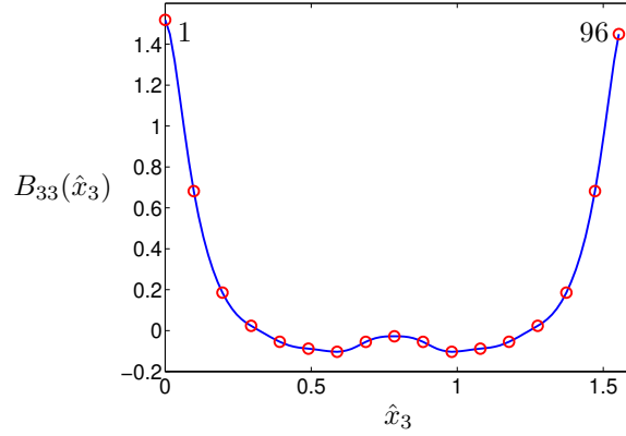
Figure S.4: Periodic two-point correlation, B_{33}(\hat{x}_3) = \langle v'_3(x_3)v'_3(x_3 + \hat{x}_3) \rangle , of DNS data in channel flow taken from [99].
