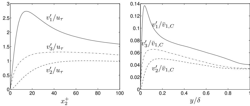
Figure 11.9: Flow between two parallel plates. Direct numerical simulations [42]. Re = \bar{v}_{1,C} \delta / \nu = 7890 . u_\tau / \bar{v}_{1,C} = 0.050 . Fluctuating velocity components v'_i = \sqrt{v_1'^2} .
