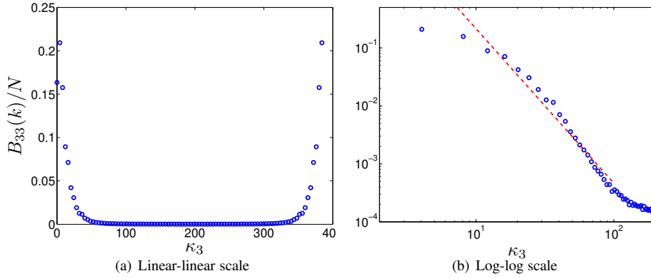
Figure S.5: The energy spectrum of \overline{v_3'^2} versus wavenumber, \kappa_3 . Dashed line in b) show -5/3 slope. Taken from [99].
