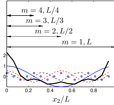
Figure 18.4: v'_2 vs. x_2/L . —: term 1 ( m = 1 ); - - : term 2 ( m = 2 ); - · - : term 3 ( m = 3 ); ○: term 4 ( m = 4 ); —: v'_2 . Matlab code is given in Section 1.3.
