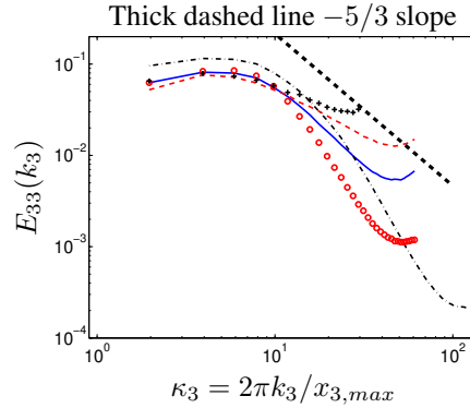
Figure 18.14: Energy spectra in fully developed channel flow [127]. \delta denotes half channel width. Number of cells expressed as (\delta/\Delta x_1, \delta/\Delta x_3) . —: (10, 20); - - -: (20, 20); - - - -: (10, 40); o: (5, 20); +: (10, 10).
