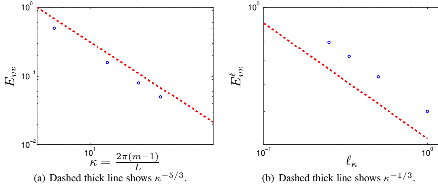
Figure I.2: Energy spectrum of v' . \circ : E_{vv} = A_m^2 . Matlab code is given in Section I.3.
