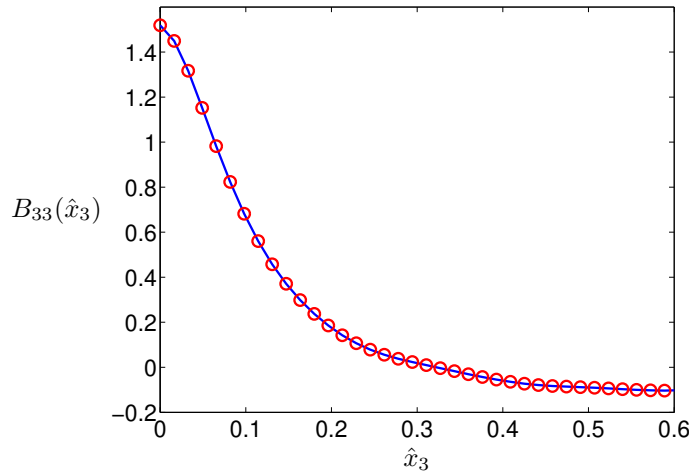
Figure S.1: Two-point correlation, B(\hat{x}_3) = \langle v'_3(x_3 - \hat{x}_3)v'_3(x_3) \rangle , of DNS data in channel flow taken from [99].
