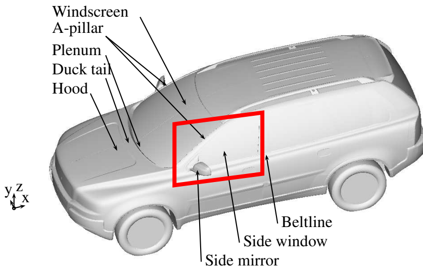
Vehicle geometry (from [115]). Red region shows embedded LES region
