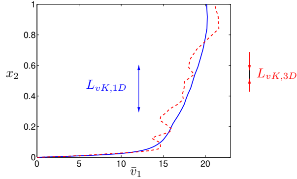
Figure 22.1: Velocity profiles from a DNS of channel flow. Solid line: time-averaged velocity with length scale L_{v,1D} , Eq. 22.1 ; dashed line: instantaneous velocity with length scale L_{vK,3D} , Eq. 22.3.
