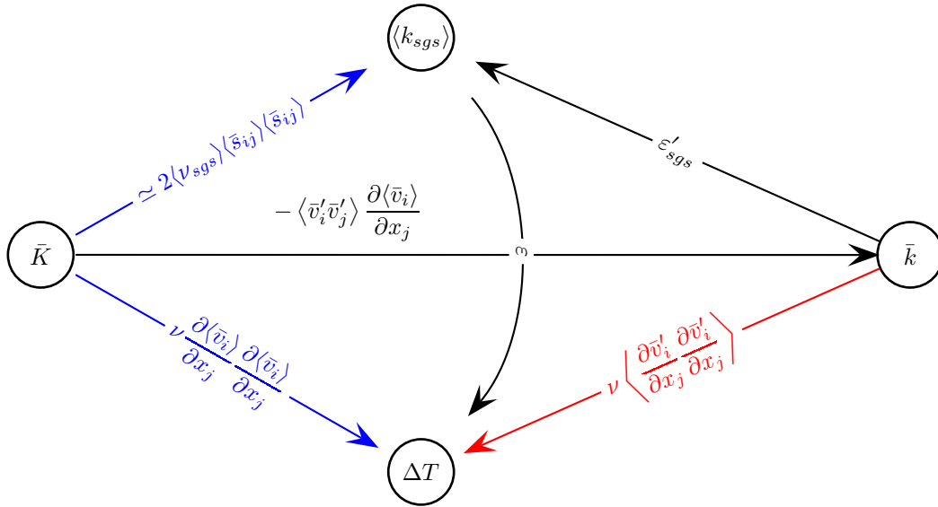
Figure R.4: Transfer of kinetic turbulent energy. \bar{K} = \frac{1}{2} \langle \bar{v}_i \rangle \langle \bar{v}_i \rangle and \bar{k} = \frac{1}{2} \langle \bar{v}'_i \bar{v}'_i \rangle denote time-averaged kinetic and resolved turbulent kinetic energy, respectively. \Delta T denotes increase in internal energy, i.e. dissipation. The cascade process assumes that the term in red is negligible (see also Fig. 8.2). The terms in blue show viscous and the SGS dissipation of the mean flow which is not included in the cascade process.
