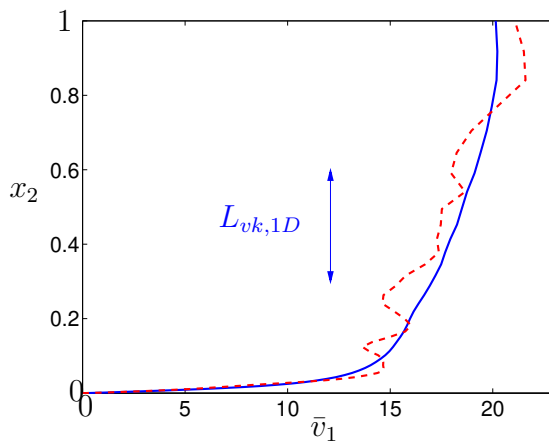
Solid line: L_{vk,1D} ; dashed line: L_{vk,3D}
