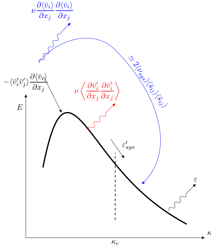
Figure Q.4: Energy spectrum. Transfer of kinetic energy. The cascade process assumes that the term in red is negligible (see also Fig. 8.2). The terms in blue show viscous and the SGS dissipation of the mean flow which is not included in the cascaded process.
