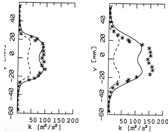
Figure 19.4: 2D URANS k - \varepsilon simulations compared with experiment [132]. Solid lines: total turbulent kinetic energy; dashed lines: resolved turbulent kinetic energy; *: experimental data. Left figure: x = 0.43H ; right figure: x = 1.1H ( x = 0 at the downstream vertical plane of the flame-holder).
