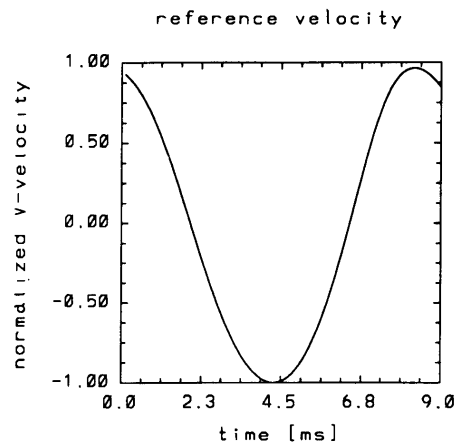
Figure 19.3: 2D URANS k - \varepsilon simulations [132]. One cycle of the \bar{v}_2 velocity in a cell near the upper-right corner of the flameholder.
