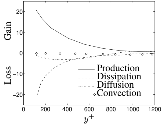
Boundary along a flat plate. Energy balance in k equation.
