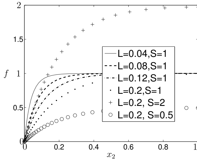
Solution of the equation L^{-1}\partial^2 f/\partial x_2^2 + S = 0 for different L and S
