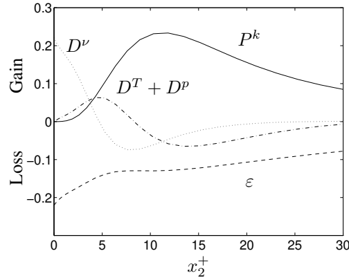
Figure 11.8: Flow in fully developed channel flow. Direct numerical simulations [42]. Re = \bar{v}_{1,C} \delta / \nu = 7890 (subscript C denotes the center of the channel). u_\tau / \bar{v}_{1,C} = 0.050 . Energy balance in k equation. Production P^k , dissipation \varepsilon , turbulent diffusion (by velocity triple correlations and pressure) D^T + D^P , and viscous diffusion D^\nu . All terms have been scaled with u_\tau^4 / \nu .
