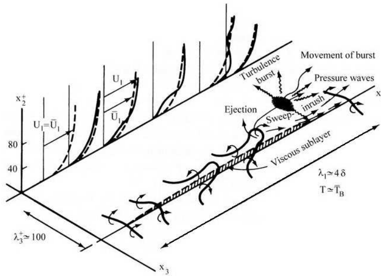
Figure 21.1: Illustration of near-wall turbulence (taken from [83]).
