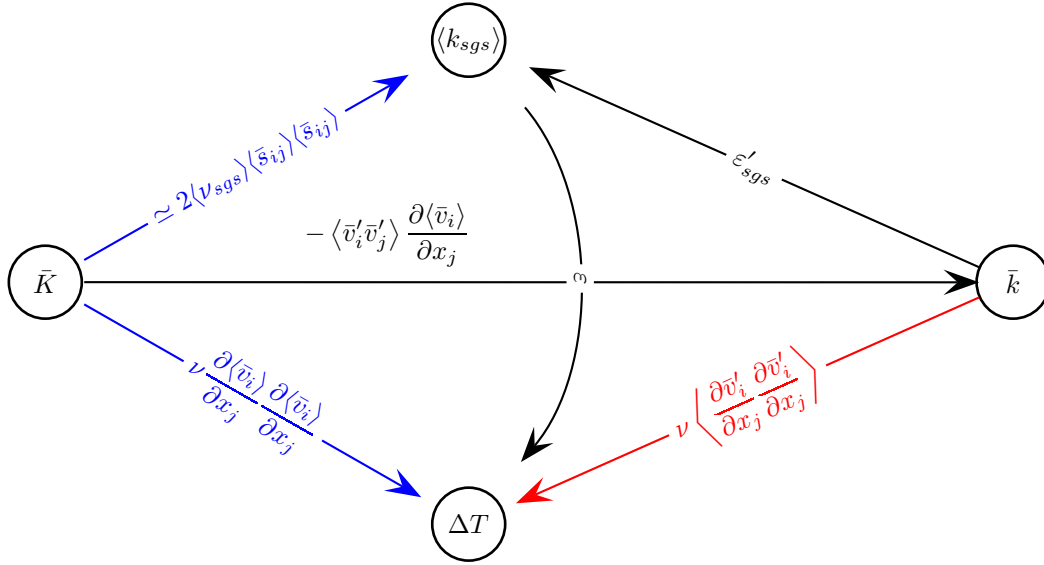
Figure Q.3: Transfer of kinetic turbulent energy. \bar{K} = \frac{1}{2} \langle \bar{v}_i \rangle \langle \bar{v}_i \rangle and \bar{k} = \frac{1}{2} \langle \bar{v}'_i \bar{v}'_i \rangle denote time-averaged kinetic and resolved turbulent kinetic energy, respectively. \Delta T denotes increase in internal energy, i.e. dissipation. The cascade process assumes that the term in red is negligible (see also Fig. 8.2). The terms in blue show viscous and the SGS dissipation of the mean flow which is not included in the cascade process.
