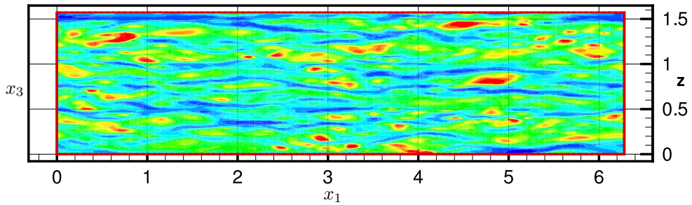
Figure 21.2: Fluctuating streamwise velocity in a wall-parallel plane at x_2^+ = 5 . DNS of channel flow [99].
