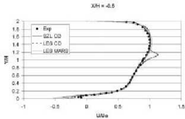
Figure 19.6: URANS simulations of the flow around a surface-mounted cube. Velocity profiles upstream the cube [133].
