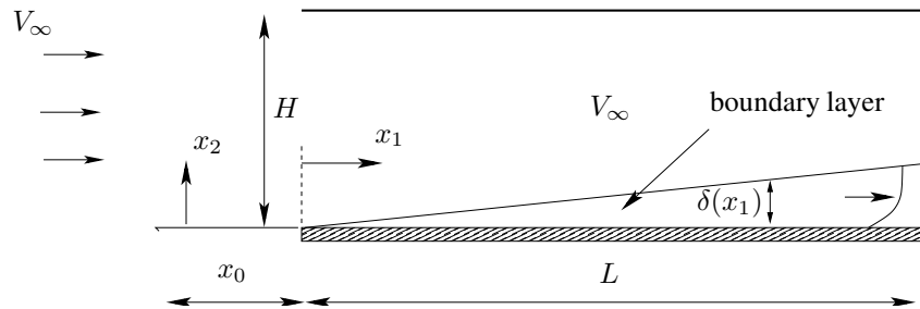
Figure E.1: Flow along a flat plate (not to scale).
