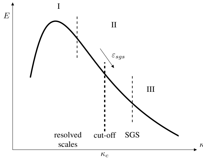
Figure Q.2: Spectrum with cut-off.
